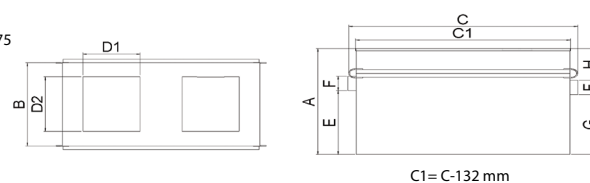
Oil separator without closing kit :
